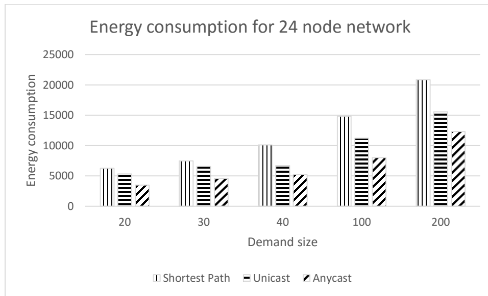
Figure 4.9 Comparison of energy consumption for 24-node network
